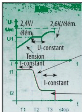
IUIa: IUIa: Constant I - constant U - constant I - turn off
