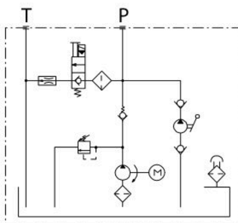
Hydraulic scheme
