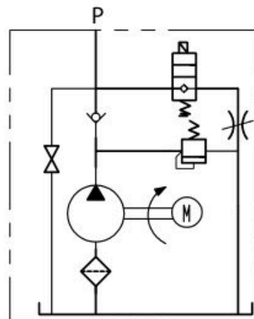
Hydraulic scheme
