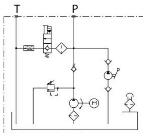
Hydraulic scheme
