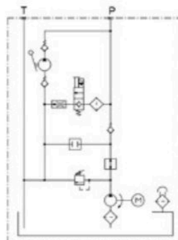
Hydraulic scheme
