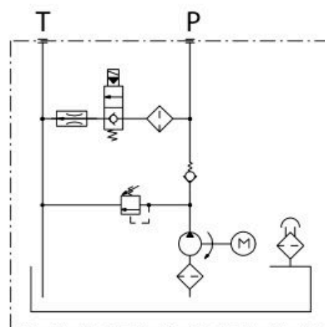
Hydraulic scheme
